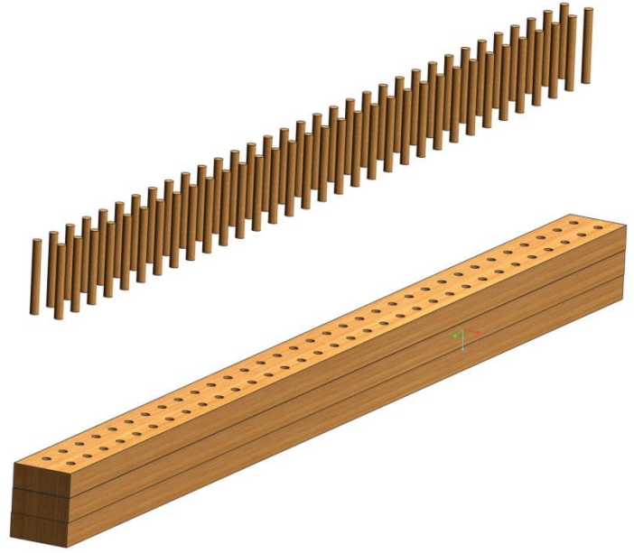
Adhesive free laminated timber beams
