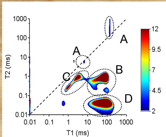
Modern wood at 65% RH
