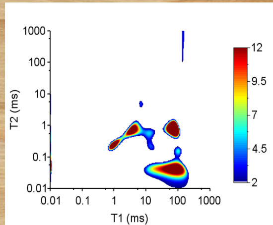
Historical wood at 65% RH
