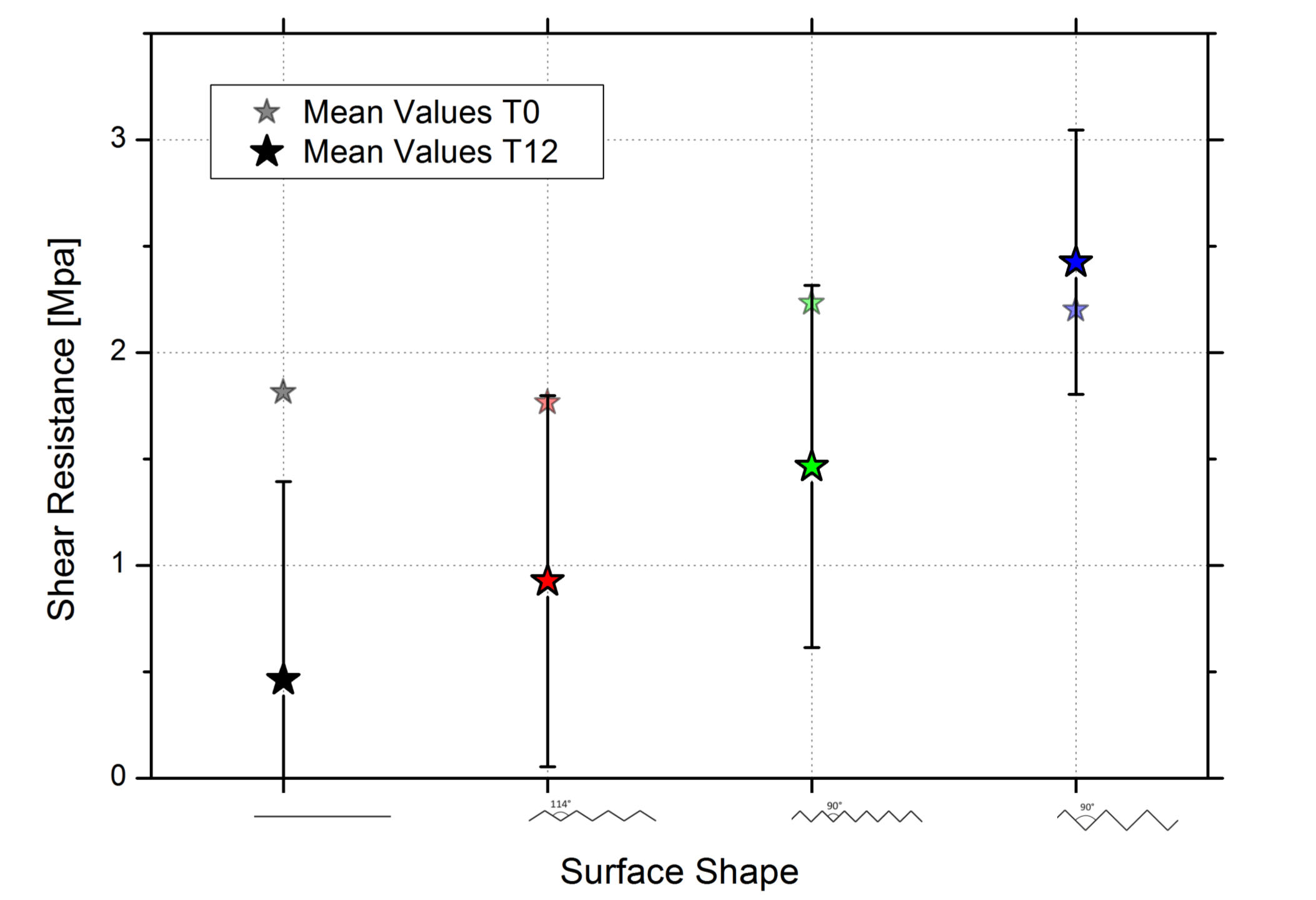
Fig. 7: Pull-out resistance of friction welded double lap joints directly after welding (T0) and after 12 climatic cycles (T12) using different surface shapes
