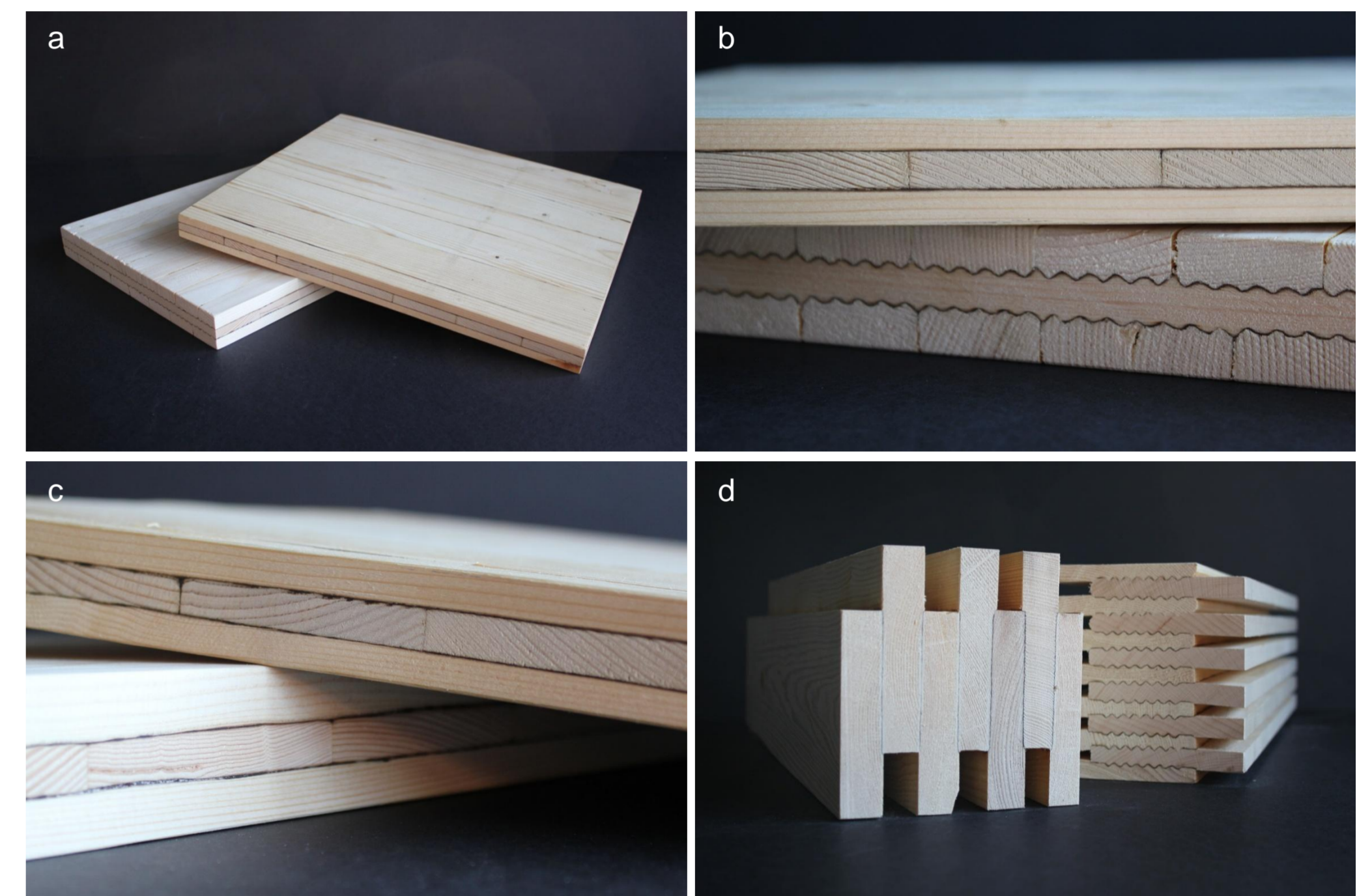
Fig. 5: First small scale prototypes of potential industrial applications of the friction welding technology in form of CLT panels and multi-layered beam and ceiling elements.
